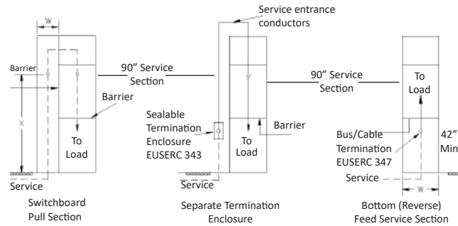
MINIMUM PULL SECTION DIMENSIONS
