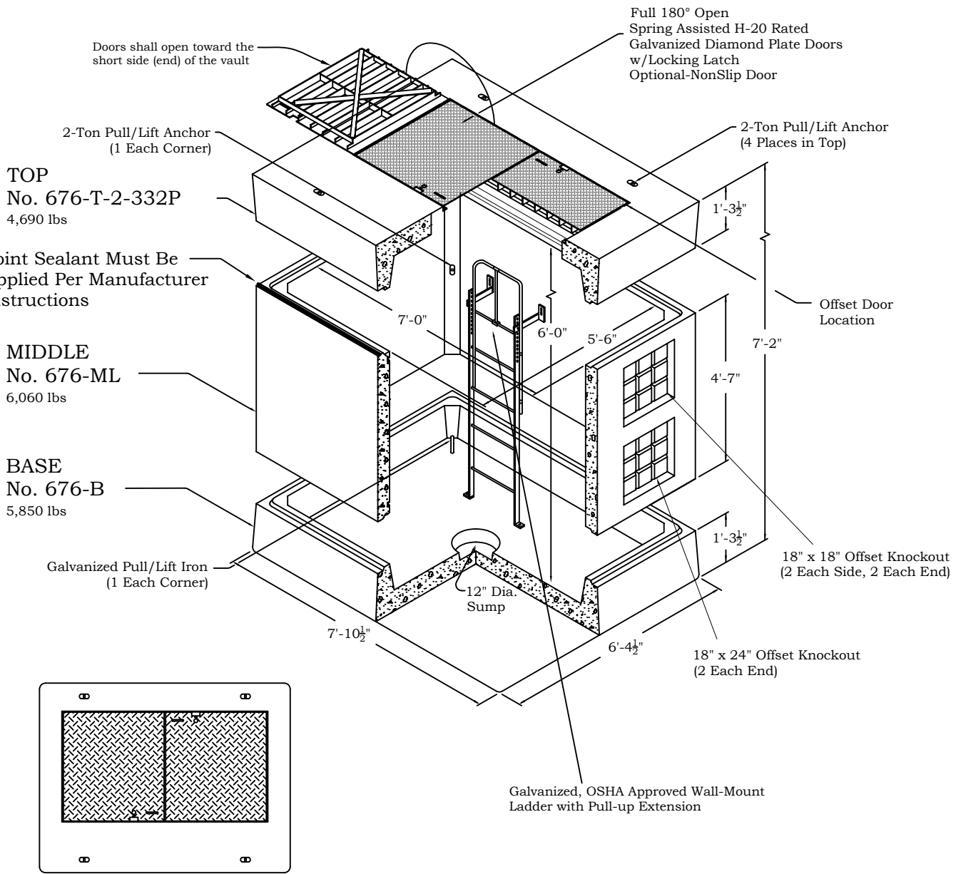
LOCKING GALV. OFFSET STEEL DOORS No. 676-T-2-332P 4,690 lbs.
